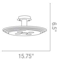
50477 Silica Semi-Flush 4Lt x 40w Halogen 120v JCD (G-9 Base) Finish CH Glass CCL CETL Dry
