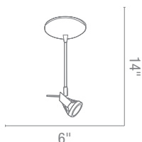
3021 era | Wall mountable Spotlight 1Lt x 0w | 12-16" (E-12) Base Finish BC C Included Shade CE L r
